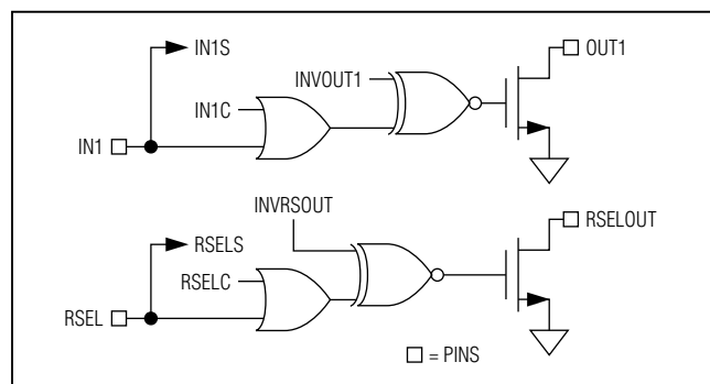
Figure 10. Logic Diagram 2
